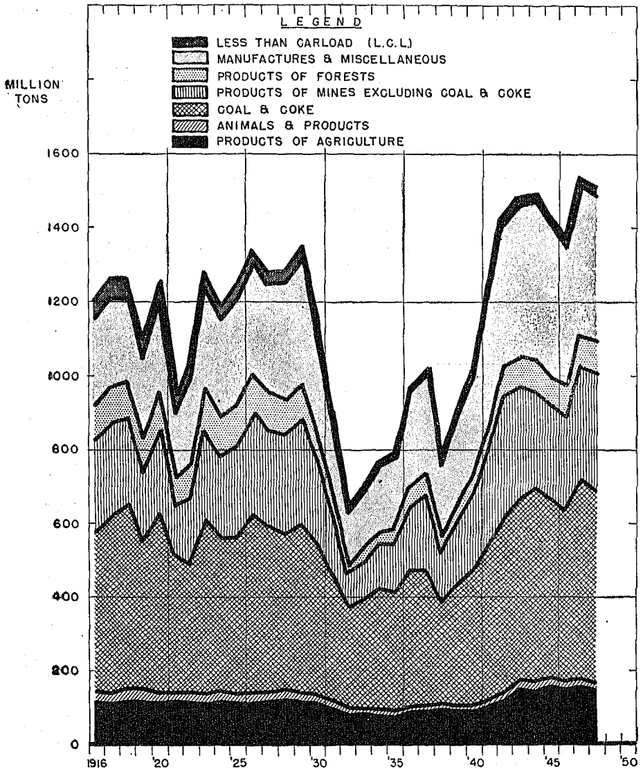
FIGURE S.—REVENUE FREIGHT ORIGINATED, CLASS I RAILROADS: 1916 TO 1948
